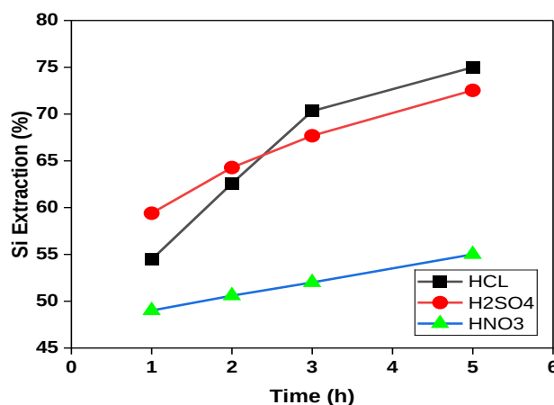
Figure 5: Si extracted from sub-75 µm heat-activated (630 °C, 4h) Lizardite
